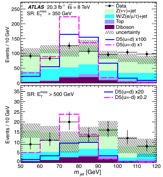
FIG. 3 (color online). Distribution of m_{\text{jet}} in the data and for the predicted background in the signal regions (SR) with E_T^{\text{miss}} > 350 GeV (top) and E_T^{\text{miss}} > 500 GeV (bottom). Also shown are the combined mono- W -boson and mono- Z -boson signal distributions with m_\chi = 1 GeV and M_* = 1 TeV for the D5 destructive and D5 constructive cases, scaled by factors defined in the legends. Uncertainties include statistical and systematic contributions.
