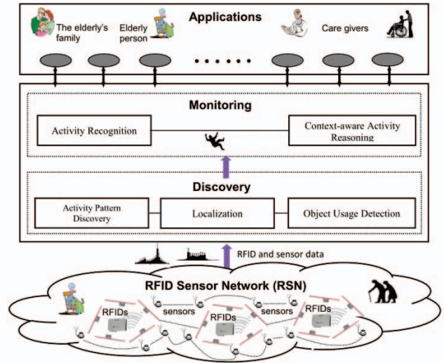
Fig. 1: The overall conceptual framework of the proposed system
