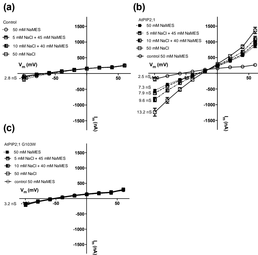
Figure 5. AtPIP2.1 \text{Na}^+ conductance is \text{Cl}^- dependent, and abolished by G103W substitution. Current-voltage curves (steady state) for (a) water injected controls ( n = 4 , mean conductance shown for all solutions at the left of the curve), (b) AtPIP2;1 ( n = 18 ) and (c) AtPIP2;1 G103W ( n = 10 , common conductance shown) in a range of \text{Cl}^- concentrations with constant \text{Na}^+ concentration, pH 7.5. Conductances shown are for the linear part of curve through the reversal potential. Mean \pm SEM.
