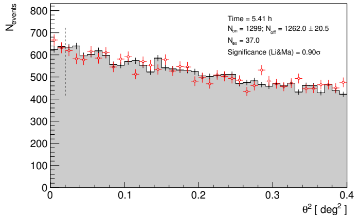
Fig. 1. Distribution of the squared angular distance, \theta^2 , after 5.41 h of observation between the reconstructed arrival direction of the gamma-ray candidate events and the position of the source in the camera (red empty circles). The \theta^2 distribution of the background events (black points) is also displayed. The vertical dashed line at \theta^2 = 0.02 \text{ deg}^2 defines the expected signal region.
