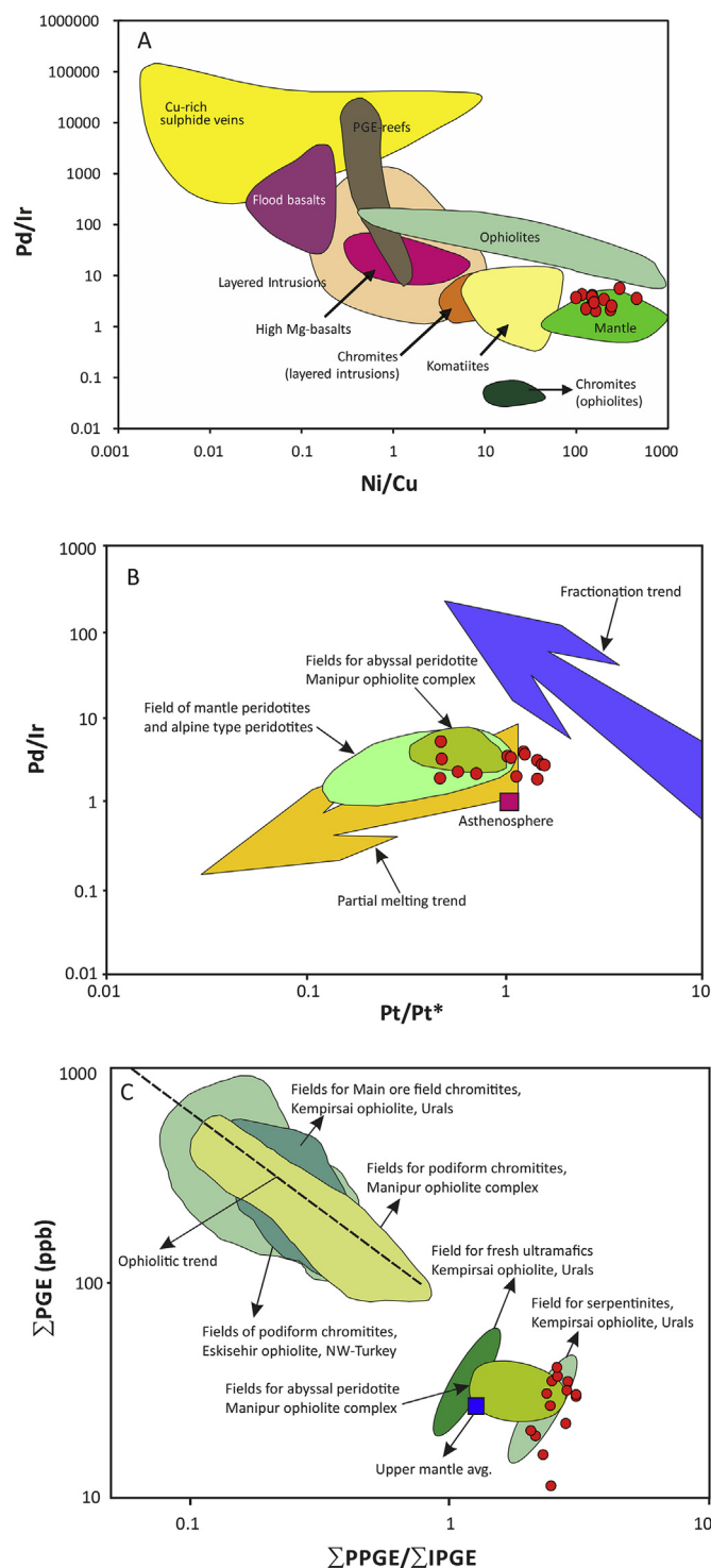
Figure 10. (A) Pd/Ir vs. Ni/Cu diagram showing the plots of mantle peridotite occupying the fields of mantle. Fields are after Barnes, 1990. (B) Pt/Pt* vs. Pd/Ir plots for the studied mantle peridotite. Fractionation and partial melting trends are from Garuti et al. (1997). Fields for mantle peridotite and alpine type peridotite (Garuti et al., 1997) and peridotites from Manipur ophiolite belt (Singh, 2013) are also shown. (C) Chondrite-normalized PPGE/IPGE vs. \Sigma PGE plot for south Andaman mantle peridotites. Upper mantle values and ophiolitic trend are from Leblanc (1991) and Melcher et al. (1999) respectively. For comparison, fields for podiform chromitites and peridotites from the Manipur Ophiolite Complex (Singh et al., 2013; Singh, 2013); main ore field chromitites, Kempirsai ophiolite massif, Urals (Melcher et al., 1999), podiform chromitites, Eskisehir ophiolite NW-Turkey (Uysal et al., 2009) are shown.
