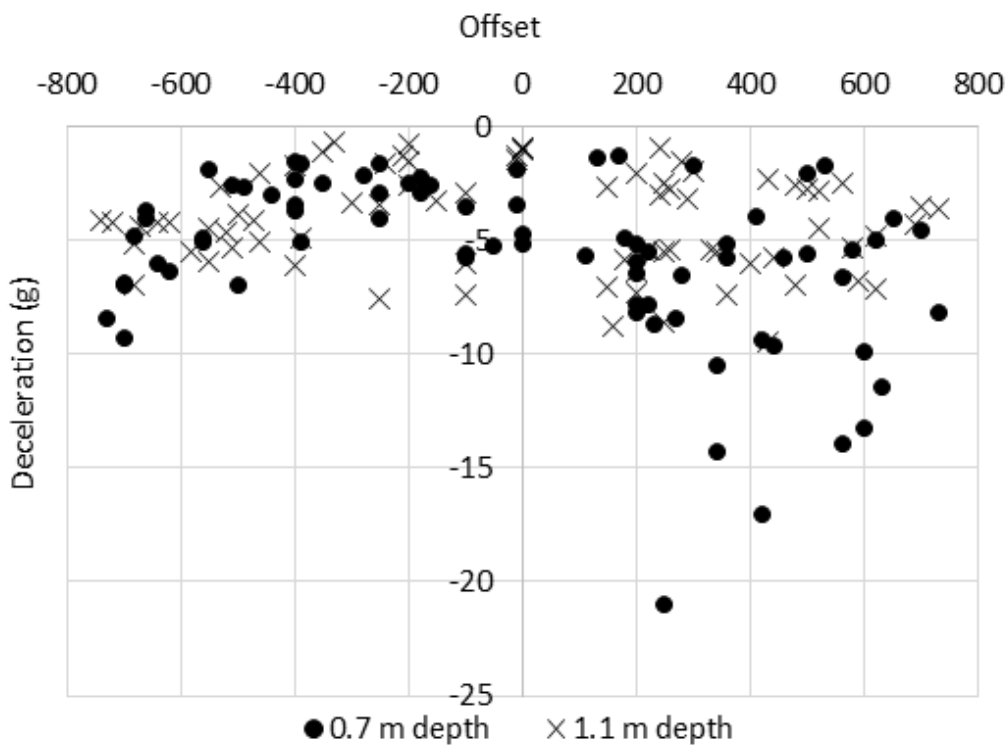
Figure 11. Distribution of peak deceleration with offset distance.
