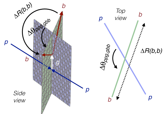
FIG. 2. Schematic diagrams illustrating the \Delta R(b, b) and \Delta\theta_{ppg, gbb} observables. In this example, the gluon is emitted at \eta = 0 .
