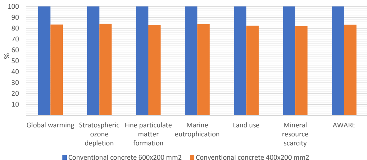
Figure 12. Comparing main Conventional Concrete wall to the reduced steel and concrete version.
