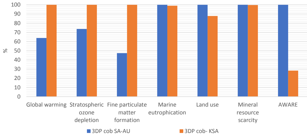
Figure 15. Comparison of 3DP Cob method in South Australia to 3DP Cob in Saudi Arabia.
