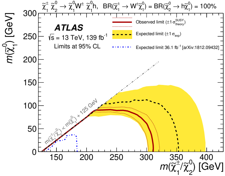
Figure 10. The observed (solid line) and expected (dashed lines) exclusion limit contours at 95% CL for the \tilde{\chi}_1^\pm \tilde{\chi}_2^0 production in the m(\tilde{\chi}_1^\pm / \tilde{\chi}_2^0) - m(\tilde{\chi}_1^0) plane. The dotted lines represent the \pm 1\sigma theoretical uncertainty for the observed limit. The \pm 1\sigma expected exclusion limit contour is shown as the shaded band. The expected limit for the 36.1 \text{ fb}^{-1} analysis [32] is also shown for comparison in the dash-dotted line.
