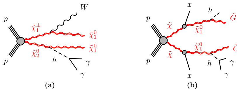
Figure 1. Signal diagrams illustrating (a) \tilde{\chi}_1^\pm \tilde{\chi}_2^0 production, and (b) a higgsino production mode from a GMSB model: \tilde{\chi}_1^0 \rightarrow h\tilde{G} . For \tilde{\chi}_1^\pm \tilde{\chi}_2^0 production, the lightest chargino ( \tilde{\chi}_1^\pm ) and next-to-lightest neutralino ( \tilde{\chi}_2^0 ) are nearly mass degenerate. In the higgsino models, the two lightest neutralinos, \tilde{\chi}_1^0 and \tilde{\chi}_2^0 , and the lightest chargino \tilde{\chi}_1^\pm are approximately mass degenerate, and the \tilde{\chi}_1^0 is the lightest of the four nearly degenerate higgsino states, x is the particle with low momentum from the promptly decay of \tilde{\chi}_1^\pm and \tilde{\chi}_2^0 .
