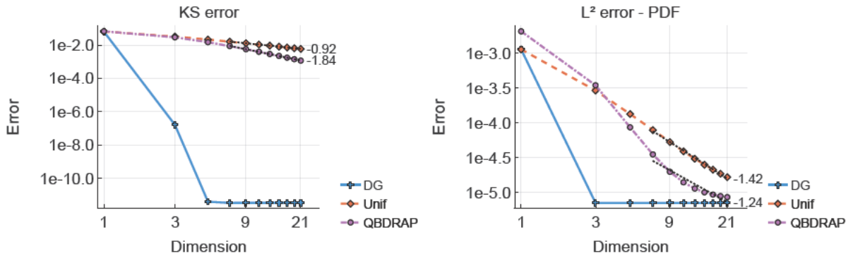
Figure 7.23: KS error (left) and L^2 error of the PDF (right) for Model 7.13 using the DG (blue solid line), uniformisation (orange dashed line) and QBD-RAP (purple dotted line) schemes. The black dotted lines are linear least-squares fits to the last 8 data points and the slopes of the least square lines are written next to the last point.
