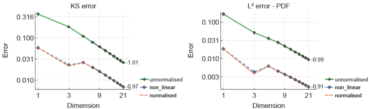
Figure 7.2: KS error (left) and L^2 error of the PDF (right) of Example 7.2 for the three closing vectors considered; unnormalised (green solid line), non-linear normalised (blue dashed line) and normalised (orange dash-dotted line). The error curves of the non-linear normalised and normalised closing vectors are almost coincident. The black dotted lines are linear least-squares fits to the last 8 data points and the slopes of the least square lines are written next to the last point.
