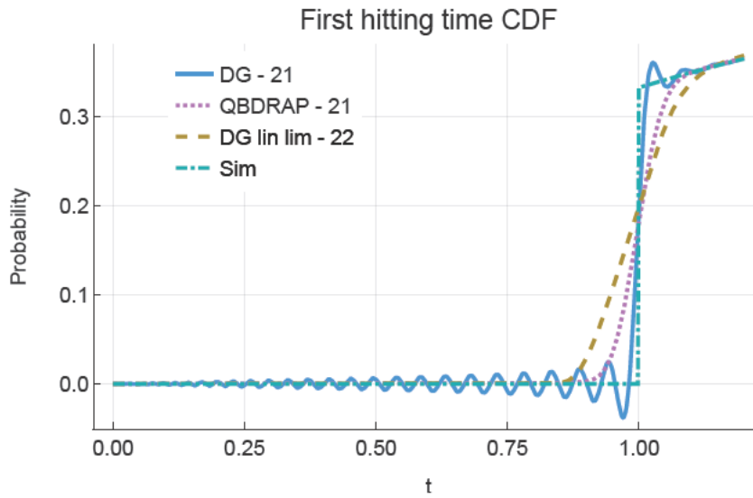
Figure 7.33: Approximations of the CDF of the first hitting time in Phase 1 for Model 7.13 with the point mass initial condition. The blue line was obtained from the dimension-21 DG scheme, the purple dotted line from the dimension-21 QBD-RAP scheme, and the gold dashed line from the dimension 22 DG-lin-lim scheme. The empirical CDF obtained via simulation is plotted as the teal dashed line. The DG scheme displays negative approximations to probabilities.
