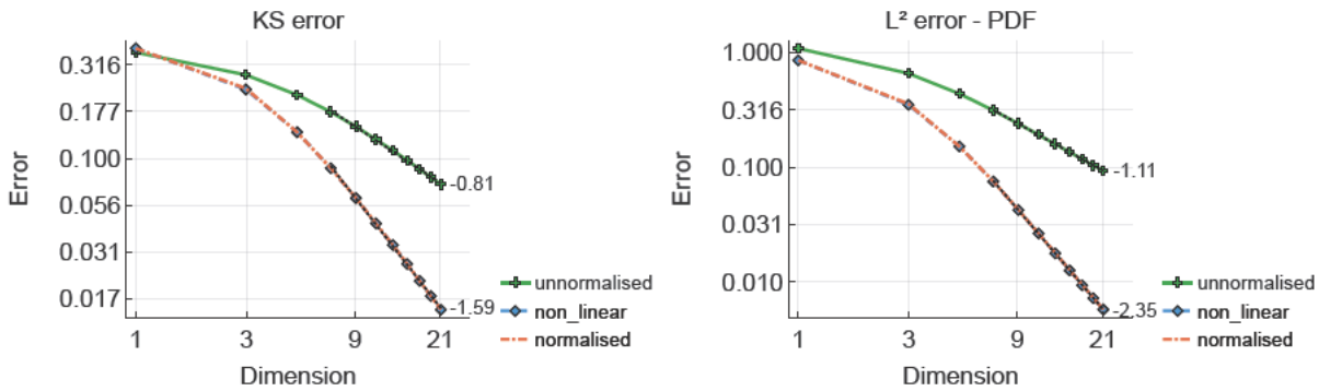
Figure 7.6: KS error (left) and L^2 error of the PDF (right) for Example 7.4 for the three closing vectors considered; unnormalised (green solid line), non-linear normalised (blue dashed line) and normalised (orange dash-dotted line). The error curves for the non-linear normalised and normalised closing vectors are almost coincident. The black dotted lines are linear least-squares fits to the last 8 data points and the slopes of the least square lines are written next to the last point.
