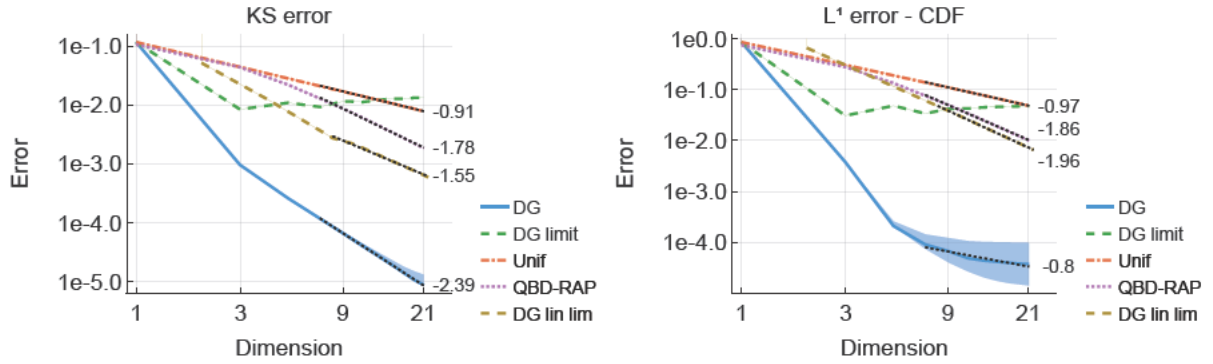
Figure 7.24: KS (left) and L^1 (right) errors between the true transient CDF at time t = 2 for Model 7.13 with the exponential initial condition, where the approximations were obtained via the DG (blue solid line), DG-lim (green dashed line), uniformisation (orange dashed line), QBD-RAP (purple dotted line) and DG-lin-lim (gold dashed line) schemes. Bootstrapped 90% confidence intervals are shown by the lighter coloured strip surrounding the lines. The black dotted lines are linear least-squares fits to the last 8 data points and the slopes of the least square lines are written next to the last point.
