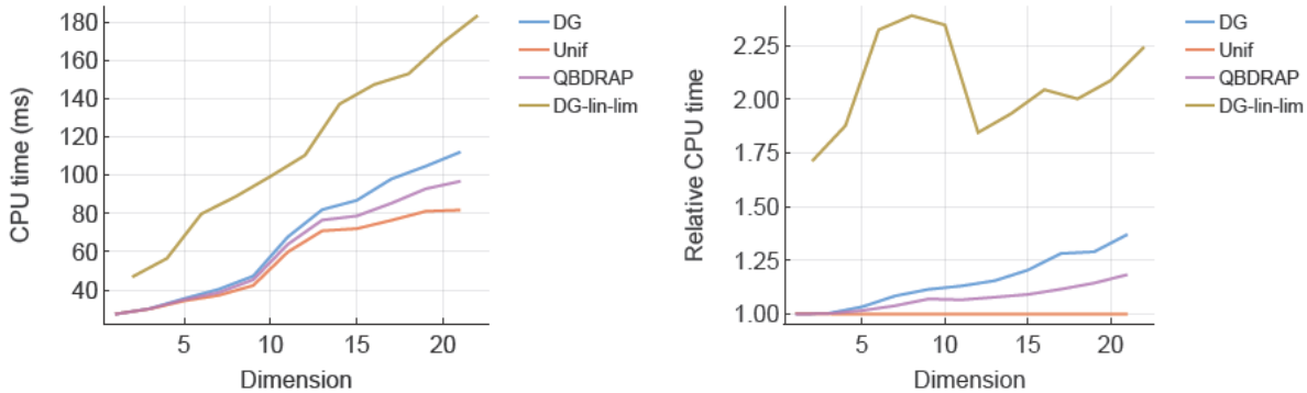
Figure 7.22: The raw (left) and relative (right) CPU time taken to integrate the approximation schemes over time to obtain the transient distributions of the travelling wave problem. The relative running time was obtained for a given dimension by dividing the running time by the running time of the fastest scheme of the same dimension (or one less in the case of the DG-lin-lim scheme).
