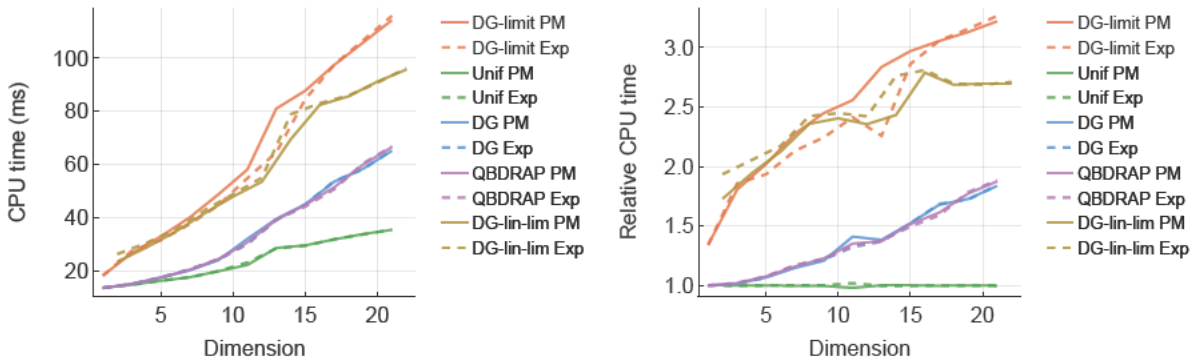
Figure 7.29: The raw (left) and relative (right) CPU time taken to integrate the approximation schemes over time to obtain the transient distributions. The running times for the point mass and exponential initial conditions are marked by the solid and dashed lines, respectively. The CPU times were obtained by running each scheme multiple times and taking the minimum CPU time. The relative running time was obtained for a given dimension by dividing the running time for that scheme by the running time of the fastest scheme of the same dimension (or one less in the case of the DG-lin-lim scheme).
