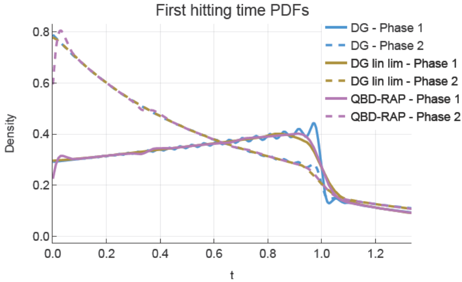
Figure 7.31: Approximations of the PDF of the first hitting time for Model 7.13 with the exponential initial condition. The blue lines were obtained from the dimension-21 DG scheme, the purple lines were obtained from the dimension-21 QBD-RAP scheme and the gold lines were obtained from the dimension 22 DG-lin-lim scheme. The DG scheme displays oscillations around the discontinuities at t = 1 . The QBD-RAP scheme has oscillations near t = 0 and t = 0.4 .
