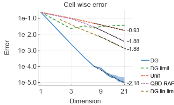
Figure 7.25: Cell-wise error metric from (7.11) for Model 7.13 with the exponential initial condition, where the approximations were obtained via the DG (blue solid line), DG-lim (green dashed line), uniformisation (orange dashed line), QBD-RAP (purple dotted line) and DG-lin-lim (gold dashed line) schemes. Bootstrapped 90% confidence intervals are shown by the lighter coloured bars surrounding the lines. The black dotted lines are linear least-squares fits to the last 8 data points and the slopes of the least square lines are written next to the last point.
