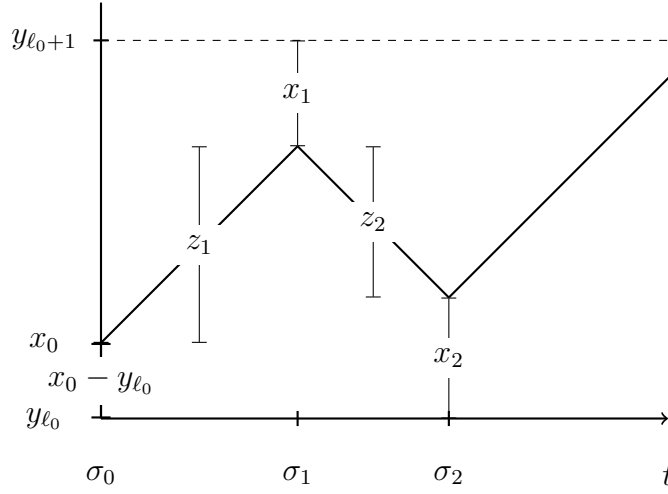
Figure 5.2: A sample path contributing to the integrand of the Laplace transform (5.35) for fixed x_1, x_2 . z_1 = \Delta - x_1 - (x - y_{l_0}) , z_2 = \Delta - x_2 - x_1 .
