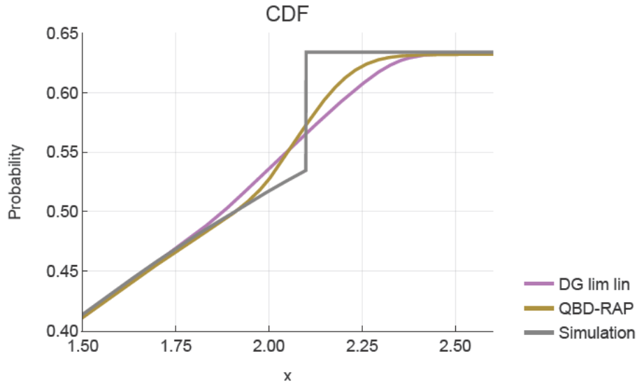
Figure 7.28: Dimension 21 QBD-RAP and dimension 22 DG-lin-lin approximations to the CDF in Phase 1 for Model 7.13 with a point-mass initial condition. An empirical estimate of the CDF obtained via simulation is plotted in grey.
