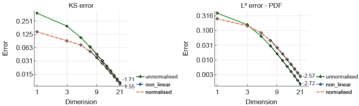
Figure 7.4: KS error (left) and L^2 error for the PDFs (right) of Example 7.3, for the three closing vectors considered; unnormalised (green solid line), non-linear normalised (blue dashed line) and normalised (orange dash-dotted line). The error curves for the non-linear normalised and normalised closing vectors are almost coincident. The black dotted lines are linear least-squares fits to the last 8 data points and the slopes of the least square lines are written next to the last point.
