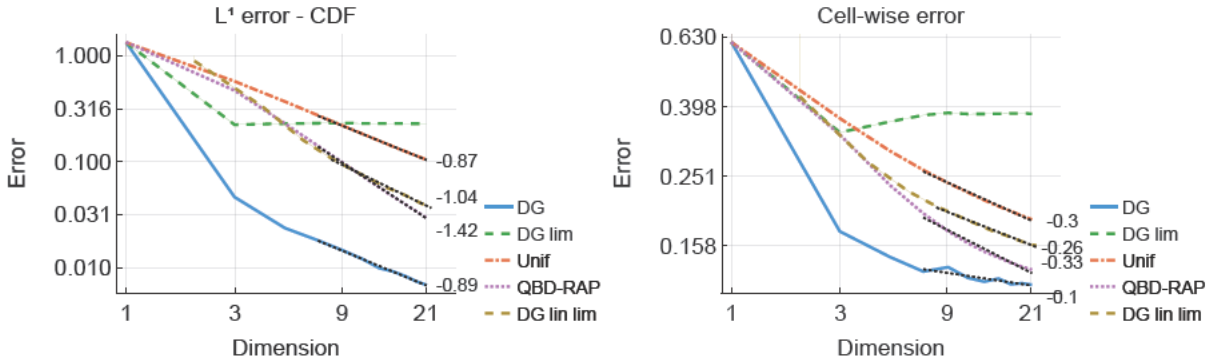
Figure 7.26: L^1 errors between the CDF, and cell-wise errors, at time t = 2 for Model 7.13 with the point-mass initial condition, where the approximations were obtained via the DG (blue solid line), DG-lim (green dashed line), uniformisation (orange dashed line), QBD-RAP (purple dotted line) and DG-lin-lim (gold dashed line) schemes. Bootstrapped 90% confidence intervals are shown by the lighter coloured bars surrounding the lines. The black dotted lines are linear least-squares fits to the last 8 data points and the slopes of the least square lines are written next to the last point.
