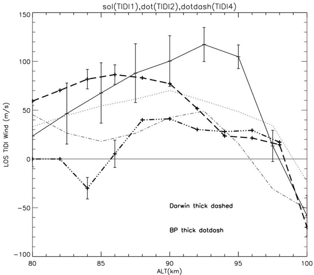
Figure 4. Line of sight (LOS) (approximately 116 degrees east of north) winds from TIDI at about 1415 UT on 31 January 2006 at three positions over central Australia. These positions, TIDI1 (13°S, 125°E), TIDI2 (20°S, 128°E), and TIDI4 (33°S, 135°E), are shown in Figure 1. Also shown are the winds from the BP (35° S, 139° E) and Darwin (12.5° S, 131° E) radars at 1400 UT. A reference line is shown at 0 m/s. Error bars are shown for the TIDI1 plot. The other TIDI errors are similar. For the radar data, representative error bars are shown for two altitudes (84 and 86 km).
