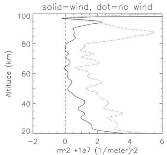
Figure 15. The m^2 from the dispersion relation for an AGW launched at an azimuth of 150 degrees east of north with a \lambda_h of 35 km and a ground-based period of 15 min. With winds (solid curve) and without winds (dotted curve). The evanescent regions, where m^2 are less than zero, are present for \lambda_h values up to about 45 km for ground-based periods of 15 min. At a \lambda_h of 30 km the evanescent region remains until ground-based periods reach around 25 min.
