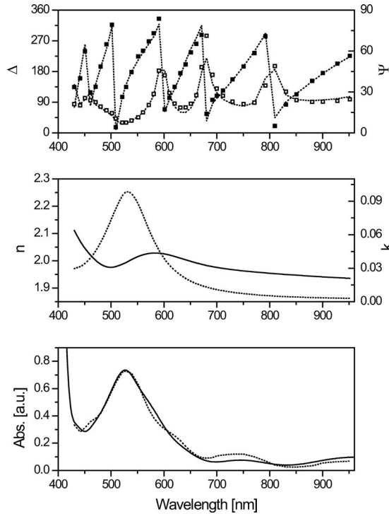
FIG. 7. Best fit for optical properties for a porous \text{TiO}_2 layer covered with D149 dye and filled with spiro-MeOTAD (607 nm) and covered with a pure spiro-MeOTAD layer (302 nm). Top: Measured \Delta (■, left axis) and \Psi (□, right axis) with the best fit to the measured data displayed (dotted lines). Middle: Refractive index (solid line, left) and extinction coefficient (dotted line, right). Bottom: UV/vis spectrum of a 302 nm mixed layer with a 187 nm layer of spiro-MeOTAD covering the surface on a quartz substrate (solid line) and the calculated absorbance (dotted line) assuming a three-layer (quartz—mixed layer—spiro-MeOTAD). The measured thicknesses are taken from profilometry and the n(\lambda)+ik(\lambda) from ellipsometry. The inset shows a blowup of the absorbance data in the transparent region of the spectrum.
