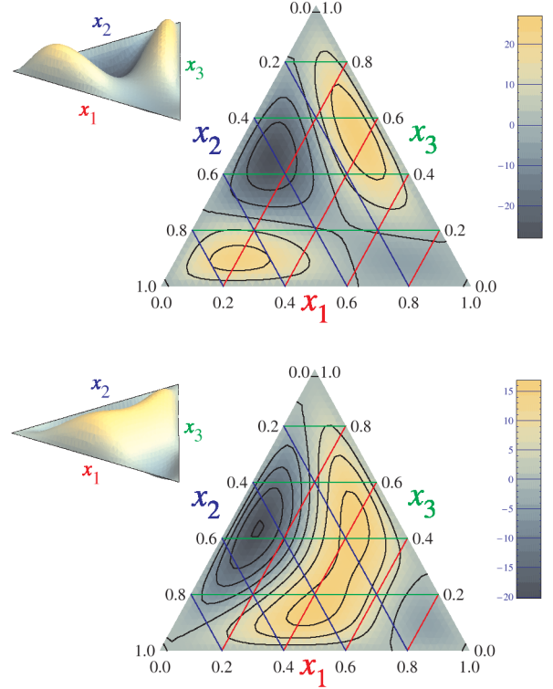
FIG. 1 (color online). Barycentric plot of the distribution amplitudes for nucleon (up) and N^*(1535) (down) at \mu_{\overline{\text{MS}}} = 1 \text{ GeV} using the central values of the lattice results. The lines of constant x_1 , x_2 , and x_3 are parallel to the sides of the triangle labeled by x_2 , x_3 , and x_1 , respectively.
