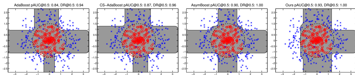
Figure 2: Decision boundaries on a toy data set with 10 weak classifiers at FPR of 0.5 The partial AUC score and detection rate at 50% false positive rate are also shown. Our approach performs best on both evaluation criteria. Our approach preserves a larger decision boundary near positive samples at \pi/4 , 3\pi/4 , -\pi/4 and -3\pi/4 angles.
