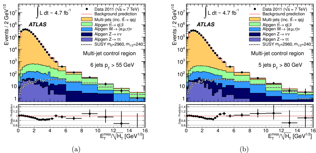
Figure 1. E_T^{\text{miss}}/\sqrt{H_T} distributions in example multi-jet control regions. (a) For exactly six jets with p_T > 55 GeV, compared to a prediction based on the E_T^{\text{miss}}/\sqrt{H_T} distribution for exactly five jets with p_T > 55 GeV. (b) For exactly five jets with p_T > 80 GeV, compared to a prediction based on four jets with p_T > 80 GeV. The multi-jet predictions have been normalized to the data in the region E_T^{\text{miss}}/\sqrt{H_T} < 1.5 \text{GeV}^{1/2} after subtraction of the predicted ‘leptonic’ backgrounds. The most important ‘leptonic’ backgrounds are also shown, based on MC simulations. Variable bin sizes are used with bin widths (in units of \text{GeV}^{1/2} ) of 0.25 (up to 4), 0.5 (from 4 to 5), 1 (from 5 to 6), and then 2 thereafter. The error bars on the data points show the Poisson coverage interval corresponding to the number of data events observed in each bin.
