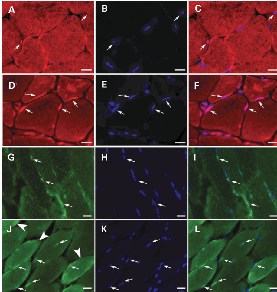
Figure 5. Immunohistochemical analysis of Myf6 and MLP reveals increased expression in nemaline muscle. Myf6 (A–F) and MLP (G–L) were detected immunohistochemically in TA muscles of 9- and 6-month-old, respectively, female WT (A–C, G–I) and NM (D–F, J–L) littermate mice. Small arrows indicate representative Myf6 containing nuclei for (A–F) and representative MLP positive nuclei for (G–L). The TA muscles from NM mice have twice as many nuclei expressing Myf6 (D–F) and four times as many MLP (J–L) containing nuclei compared with littermate controls (A–C and G–I, respectively). Furthermore, in NM mice, unlike littermate controls, increased MLP staining was observed in the cytoplasm of multiple muscle fibers [large arrow heads in (J)]. All nuclei were visualized using DAPI (stained blue in B, C, E, F, H, I, K and L). Scale bars = 16.7 \mu m.
