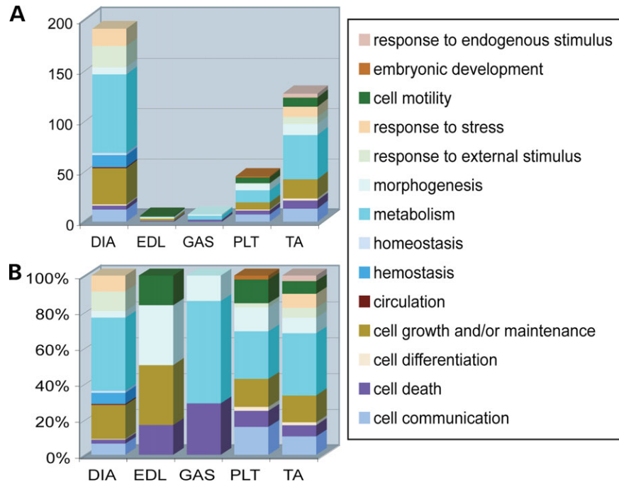
Figure 2. GO category analysis of genes considered significantly changed between WT and NM mouse muscles. All genes significantly changed in NM muscles were grouped in GO biological process categories on the basis of the function of their respective proteins. This graph shows the major GO categories implicated in each muscle studied when all significantly changed genes are considered. For DIA only, the top 200 significantly changed genes are tabulated. The results are presented as (A) the actual numbers of significantly changed probe sets in each muscle type and (B) the percent of significantly changed probe sets for each muscle type.
