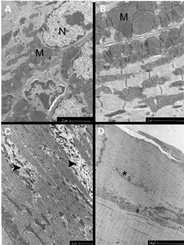
Figure 6. EM analysis of \alpha Tm_{slow}(Met9Arg) transgenic muscles reveals morphological evidence for metabolic disturbance, myofibrillar degeneration and repair in nemaline muscles. (A and B) Diaphragm of 8-month-old NM mouse: enlarged, abnormally shaped and increased numbers of mitochondria are present beneath the sarcolemma and in inter-fibrillar spaces. N, myonucleus; M, mitochondria; (C) Tibialis anterior muscle of 8-month-old NM mouse: myofibrillar degeneration is evident (arrowheads). Inter-fibrillar and subsarcolemmal mitochondria display abnormal shape, size and number. (D) Tibialis anterior muscle of 7-month-old NM mouse: localized repair is evident by the presence of an isolated, centrally localized nucleus (asterisk) within a myofiber.
