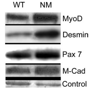
Figure 4. Western blot analysis of satellite cell markers, MyoD, desmin, Pax7 and M-Cadherin (M-Cad) (indicated at right) reveals elevations in \alpha Tm slow (Met9Arg) transgenic TA muscle from 7–8-month-old NM mice. Two to three replicate muscles from WT or NM mice were analyzed and a representative blot is shown. Control, Coomassie stained myosin light chain band.
