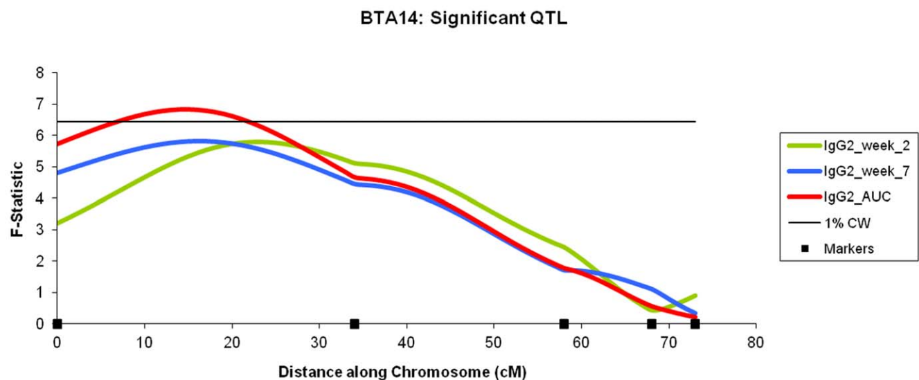
Figure 3. BTA 14: Significant QTL. F -statistic profiles for the IgG2 response elicited by the BRSV vaccine two and seven weeks post vaccination and using the AUC measurement. The constant horizontal line represents the threshold of the 1% chromosomal wide significance level ( F = 6.43 ). doi:10.1371/journal.pone.0033526.g003
