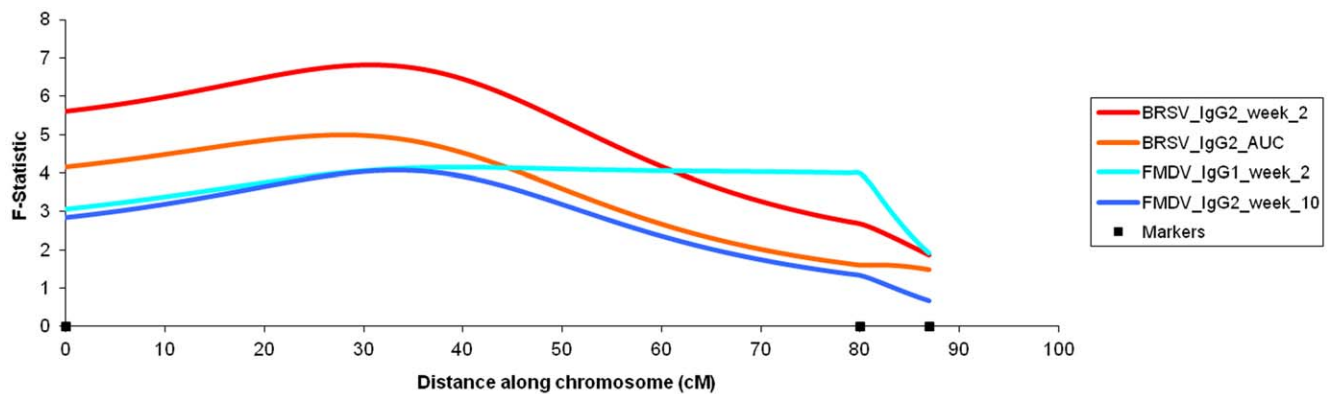
Figure 4. BTA 23: Significant QTL. F -statistic profiles for the IgG2 response elicited by the BRSV vaccine two weeks post vaccination (peak, 31; F -statistic 6.82) and the AUC measurement (peak, 27; F -statistic, 4.97) and for the IgG1 (peak, 39; F -statistic, 4.16) and IgG2 (peak, 33; F -statistic, 4.08) levels elicited by the FMDV peptide [27] 2 and 10 weeks post immunisation, respectively. doi:10.1371/journal.pone.0033526.g004
