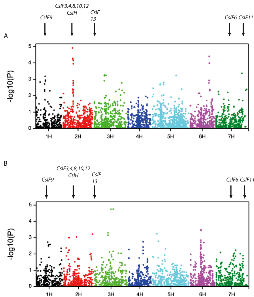
Figure 2 Manhattan plots of grain (1,3;1,4)-β-glucan content genome wide association scans (GWAS) using the Eigenstrat relationship model. The -log 10 (p-values) from a genome-wide scan are plotted against the position on each of the 7 barley chromosomes. (A) Mean Spring grain (1,3;1,4)-β-glucan content. (B) Winter grain (1,3;1,4)-β-glucan content. The positions of CslF9 on 1H, and the Csl cluster on 2H, which includes CslF3 , 4, 8, 10 and 12, are indicated by black downward arrows.
